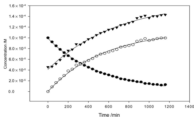
Figure 6. The concentration vs. time plots for the reaction of EuHEDTA with BNPP at pH 10.5 from HPLC analysis data. The solid lines are the best least-squares fits to the corresponding exponential curves. ●, BNPP; ○, NP; ▼, NPP. [\text{EuHEDTA}] = 10 \text{ mM} , [\text{BNPP}] = 0.10 \text{ mM} , [\text{buffer}] = 100 \text{ mM} , \mu = 0.1 \text{ M} .
