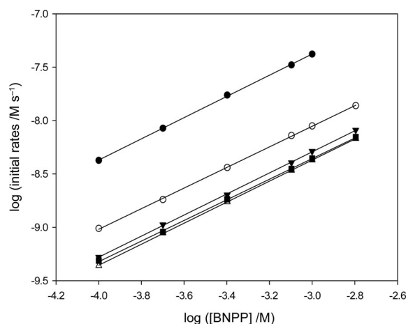
Figure 3. Plots of log (initial rates) vs. log[BNPP] for selected LnHEDTA complexes (Ln = Nd, ○; Eu, ●; Dy, ▼; Er, △; Yb, ■). [LnHEDTA] = 10 mM, [buffer] = 100 mM, [BNPP] = 0.1 mM to 1.6 mM, pH = 10.5 at 25 °C. The solid lines are the best linear least-squares fits ( R^2 \approx 1.0 ).
